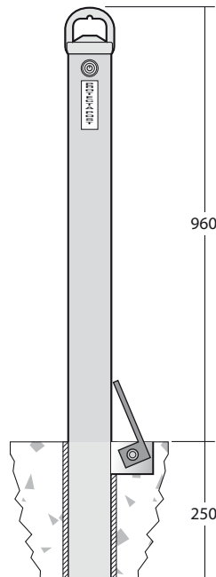
Inground sleeve with cover plate
