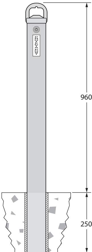
Protecta Post inground sleeve with drop in lid
